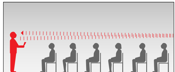
(f) Rear wall can cause a disturbing echo for speakers if over 8.5 m away. Rear wall should be absorbing or diffusing.
