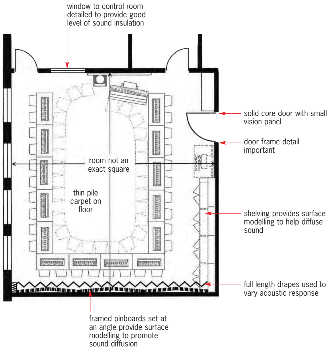
Figure 5.5: Acoustic treatment to music classroom
